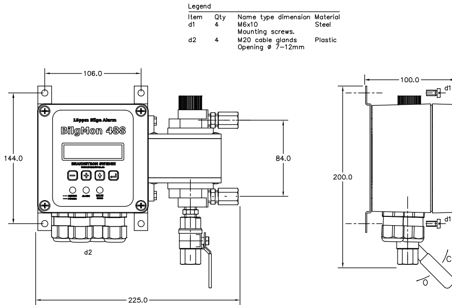
Illustration 1: Mechanical installation
