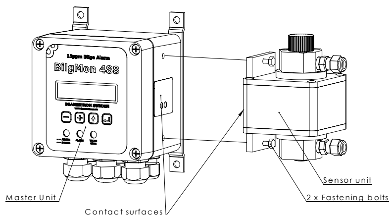
Illustration 6: Sensor unit replacement procedure.
