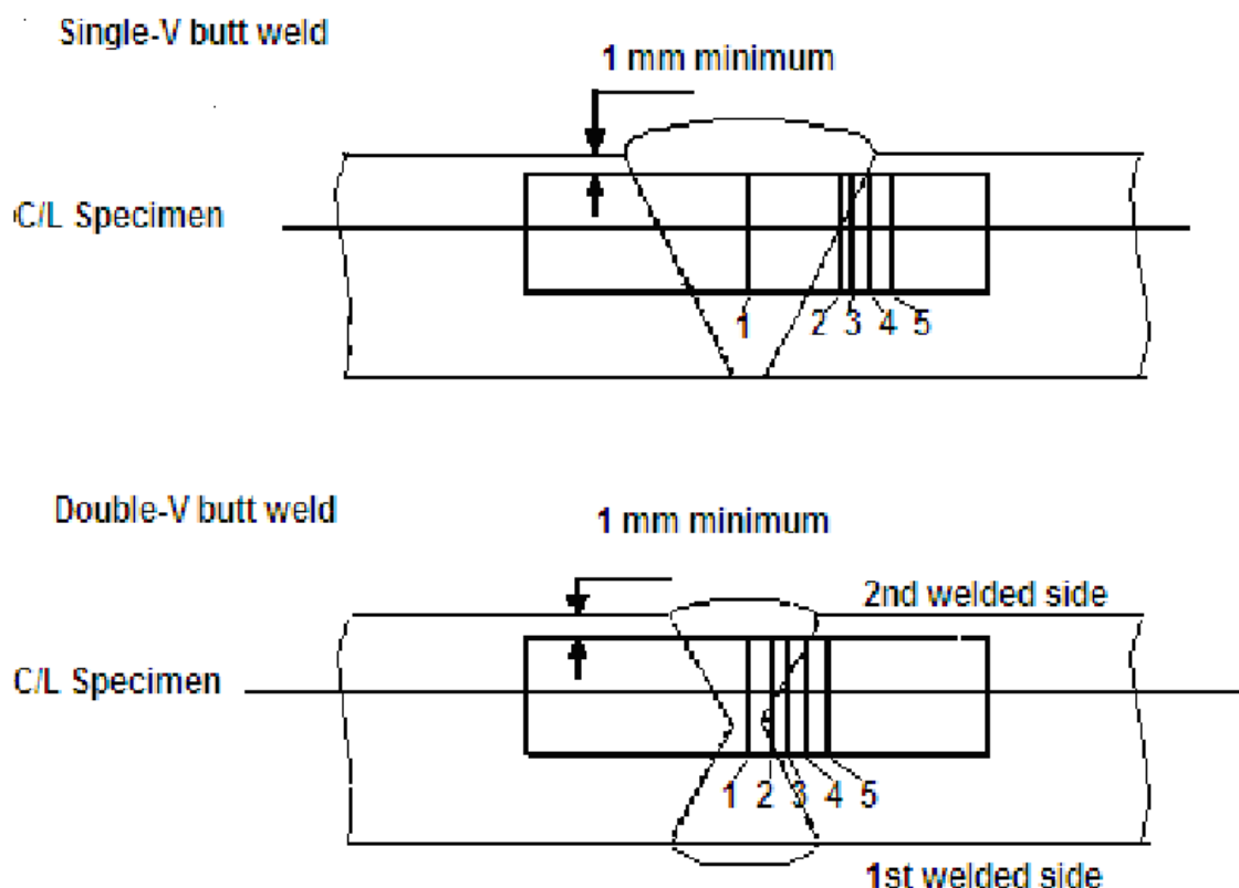
Figure 16.2 – Orientation of weld test specimen
