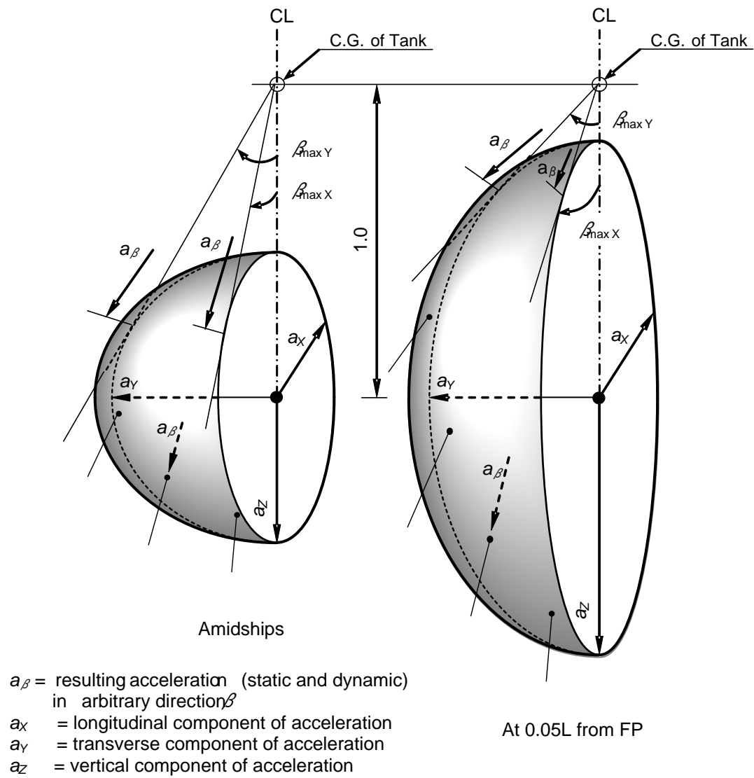
Figure 6.4.1 – Acceleration ellipsoid
