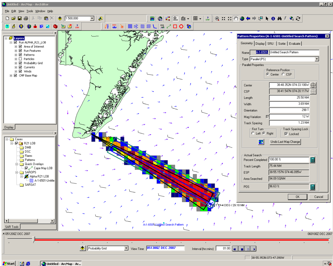
Figure 3-15 — SAROPS Search Plan for Helicopter Arriving one hour after Distress Broadcast with one hour On Scene Endurance Searching for a 20-foot Power Boat
