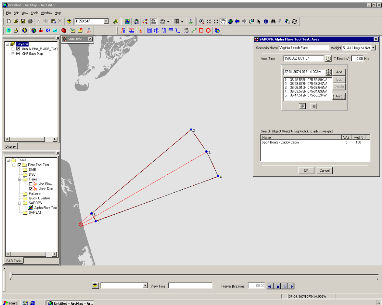
Figure I-20: Establishing SAROPS Area Scenario for a Flare Sighting
