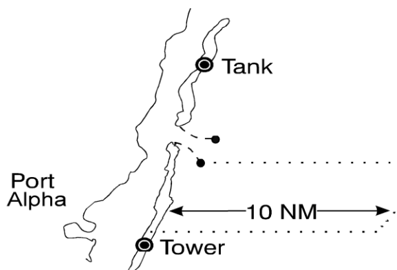
Figure H-26 Landmark Boundaries Method
