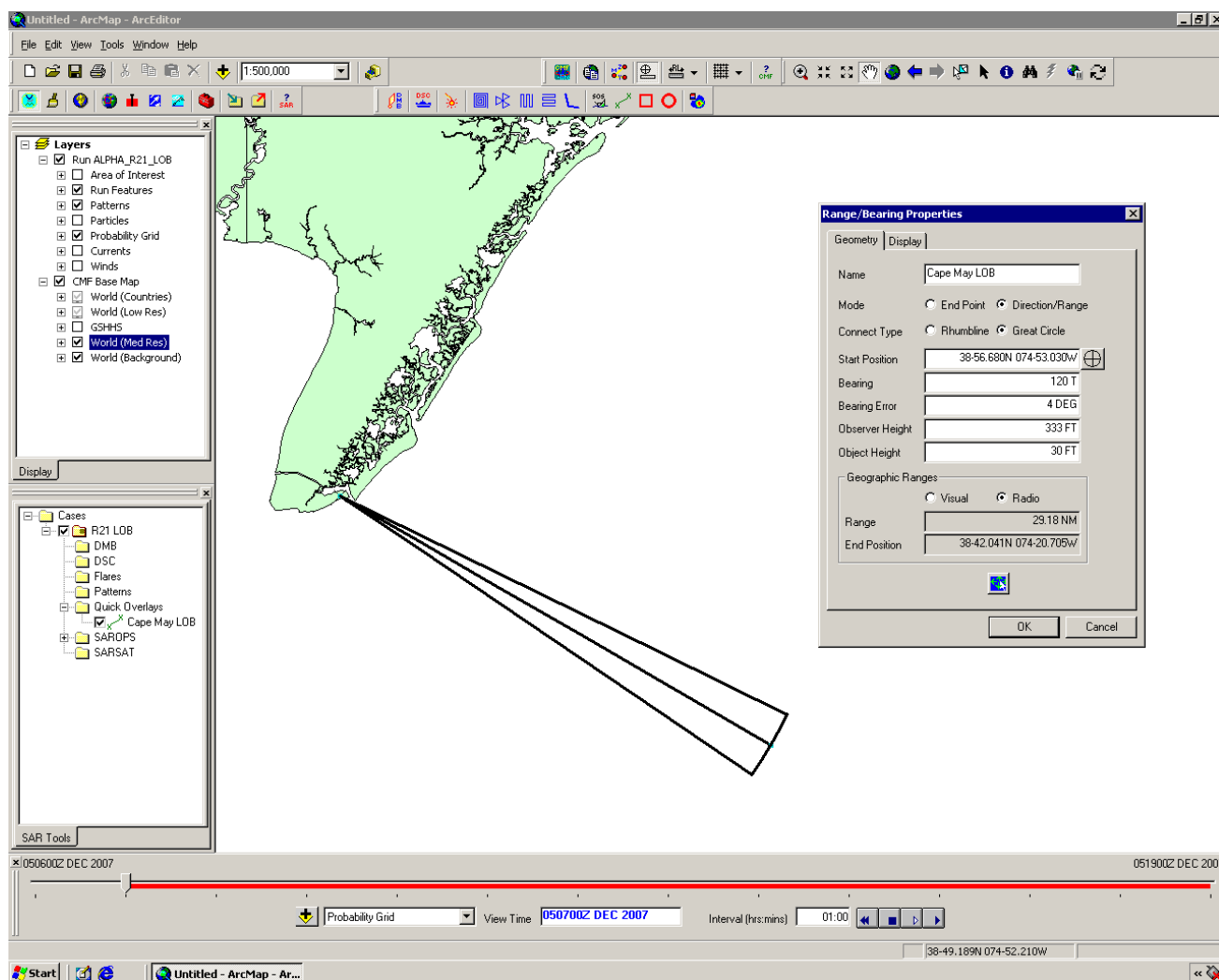
Figure 3-13 – SAROPS/SAR Tools Single LOB Range and Bearing Plot
