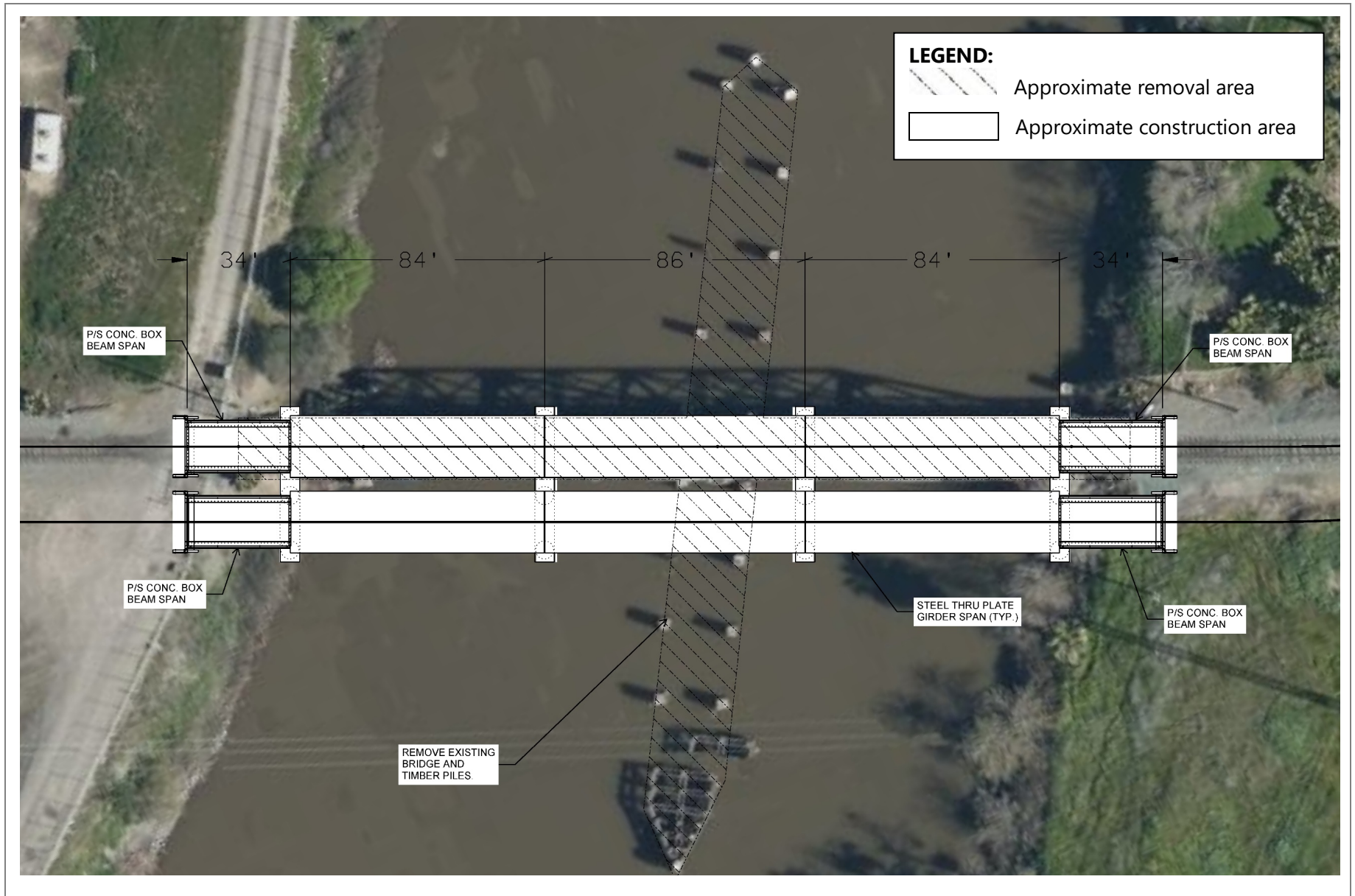
Figure 7 Proposed Rail Bridge Replacement Rail Bridge Replacement and Rail Improvements Port of Stockton, California
