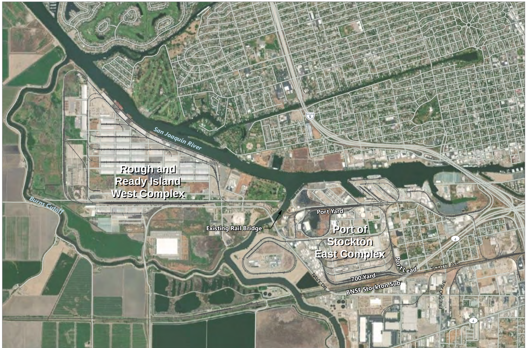
Figure 3 Existing Port Rail System Rail Bridge Replacement and Rail Improvements Port of Stockton, California
