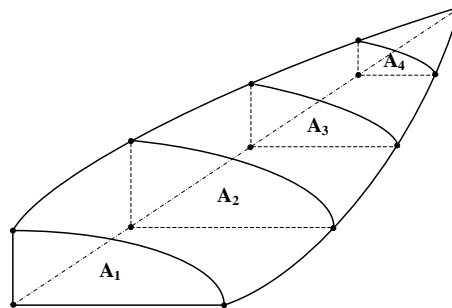
Three-dimensional Simpson's
